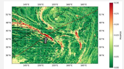
Example of turbulence forecast over the North Pacific Ocean
